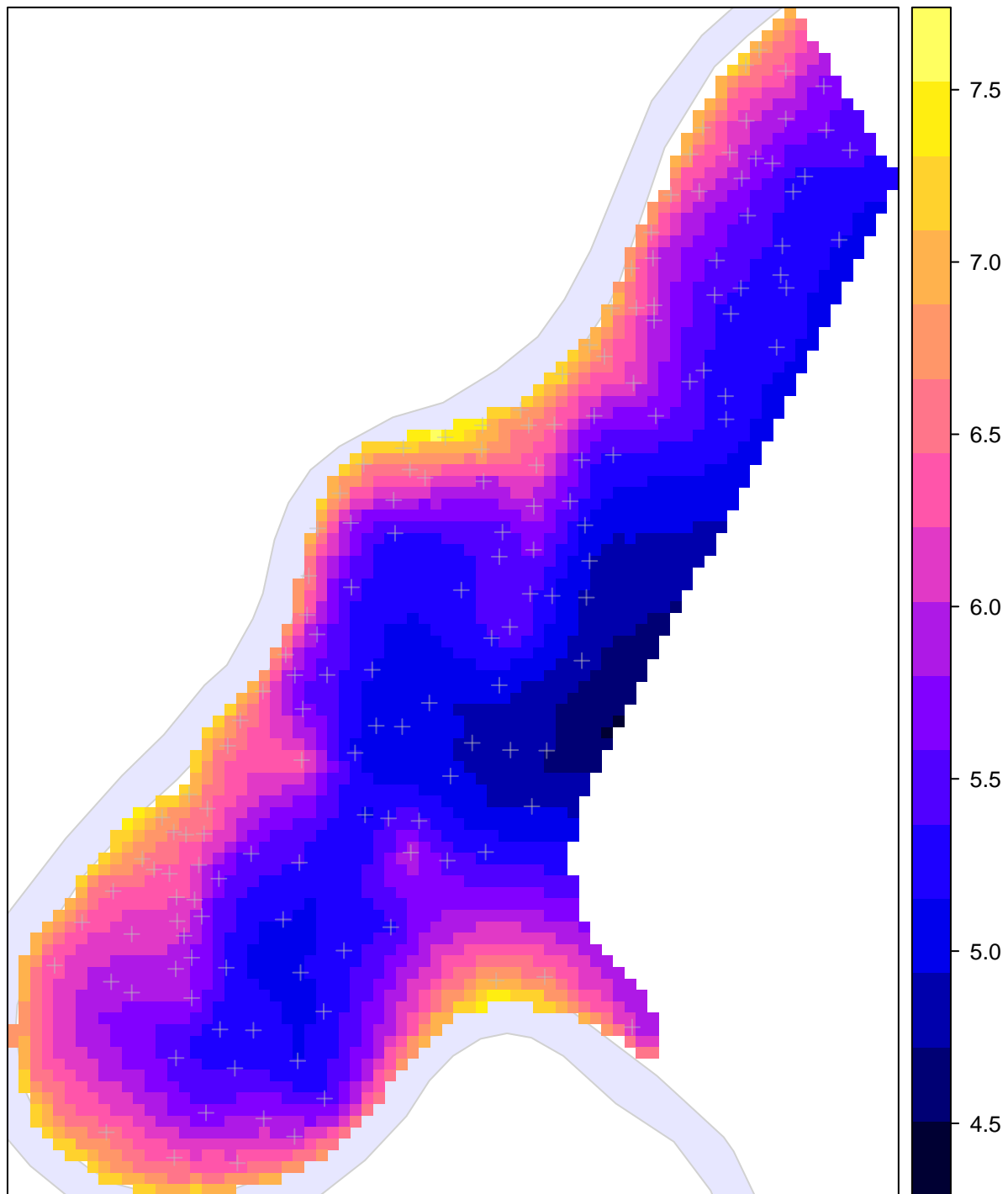
log(zinc); universal kriging using sqrt(dist to Meuse)
