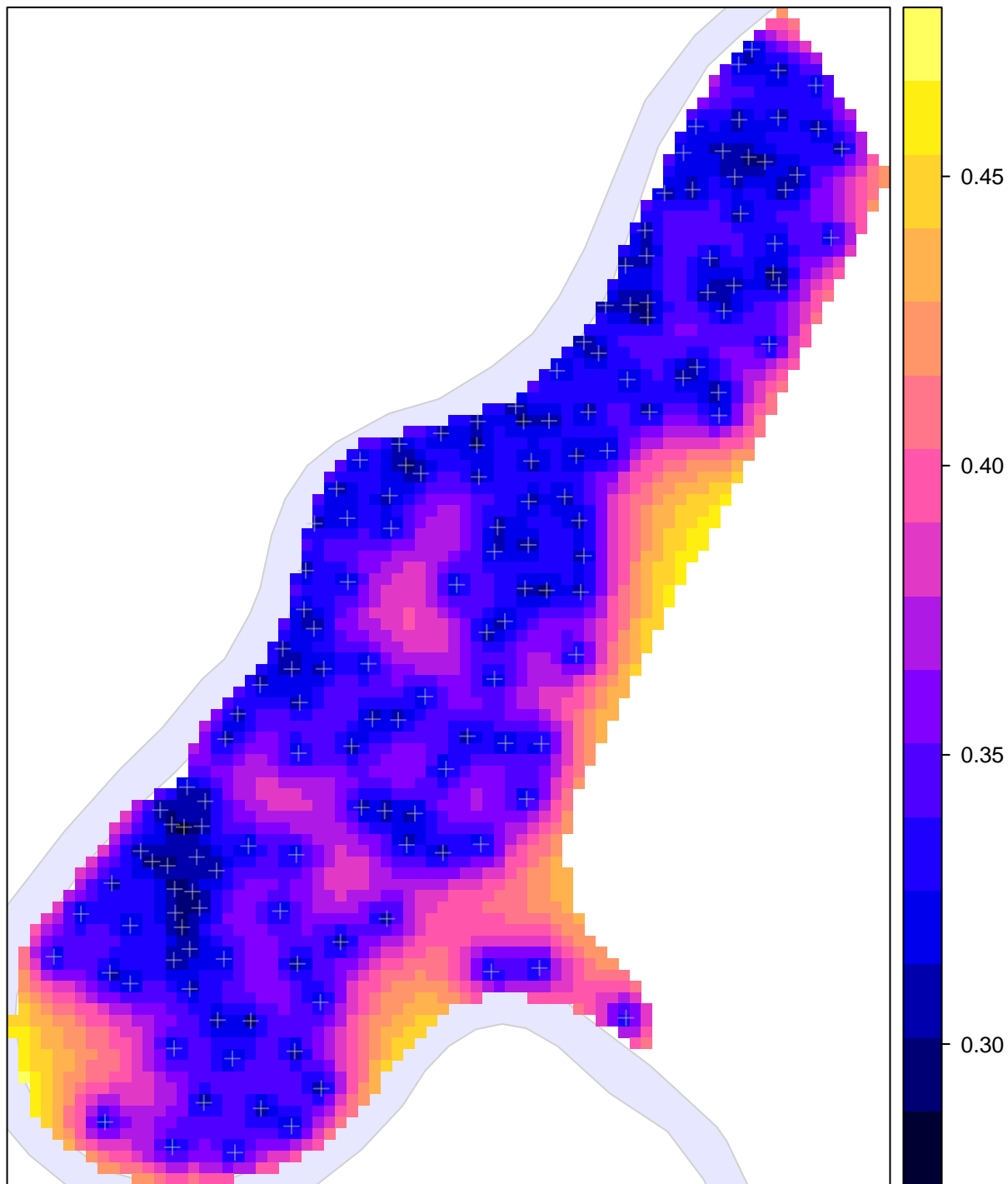
log(zinc); universal kriging standard errors
